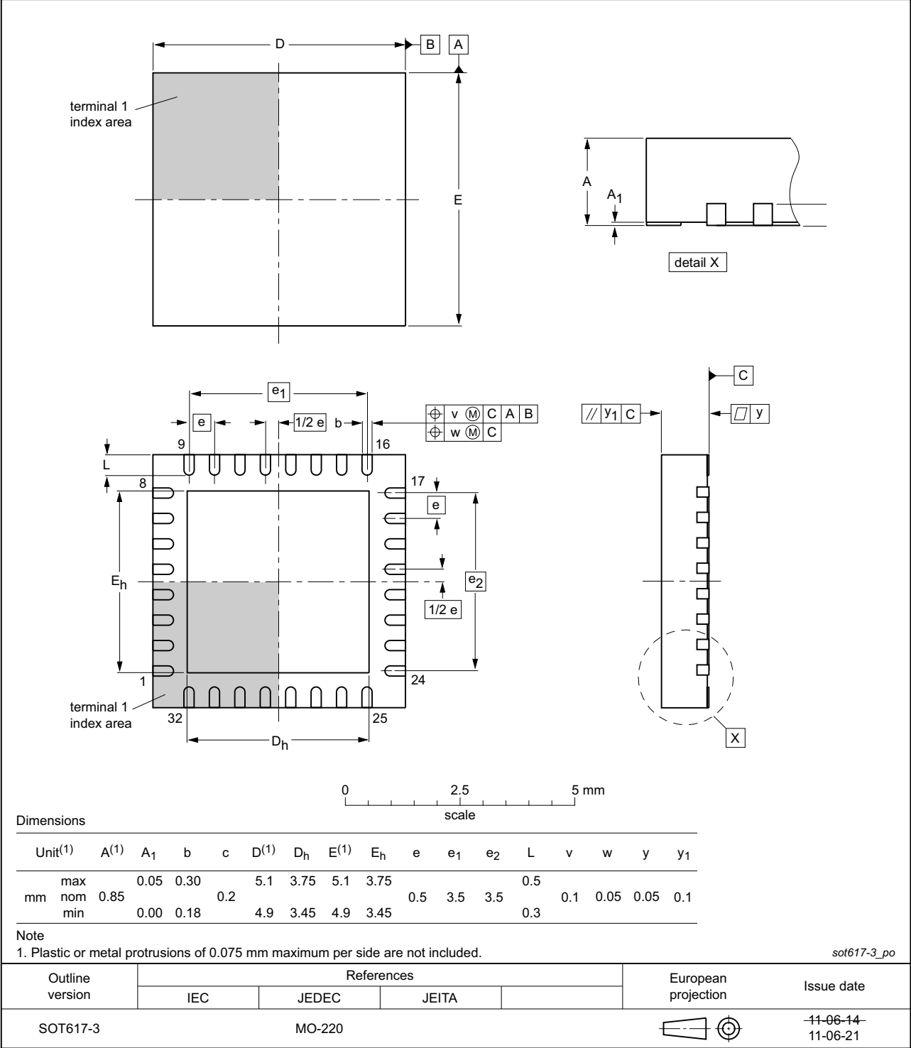
Fig 4. Package outline SOT617-3 (HVQFN32)
